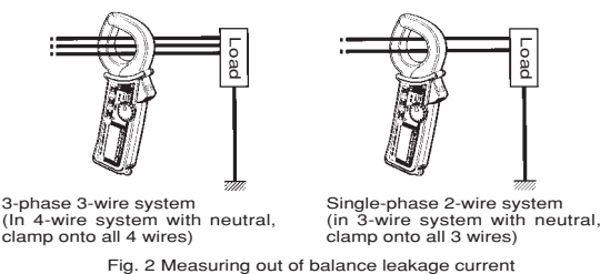
Fig. 2 Measuring out of balance leakage current
